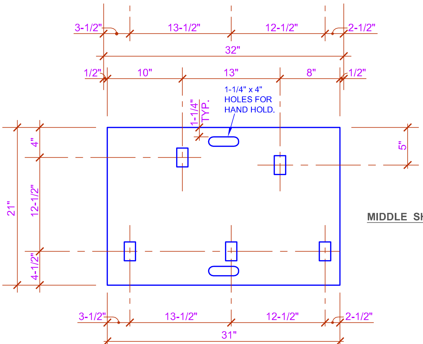
BASS BELL BOX -- Dimensions
